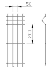
Ø5mm WIRE MESH DETAILS
