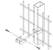
FIXING BRACKET DETAIL
